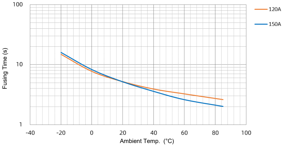
SKT-L Temp.-Time Curve
