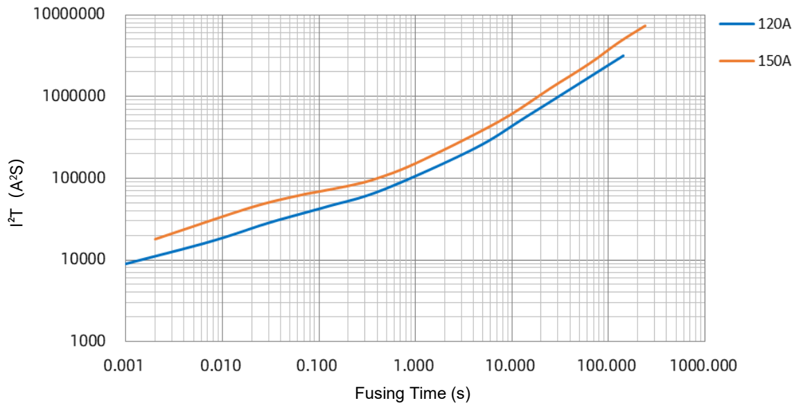
SKT-L I²t Curve
