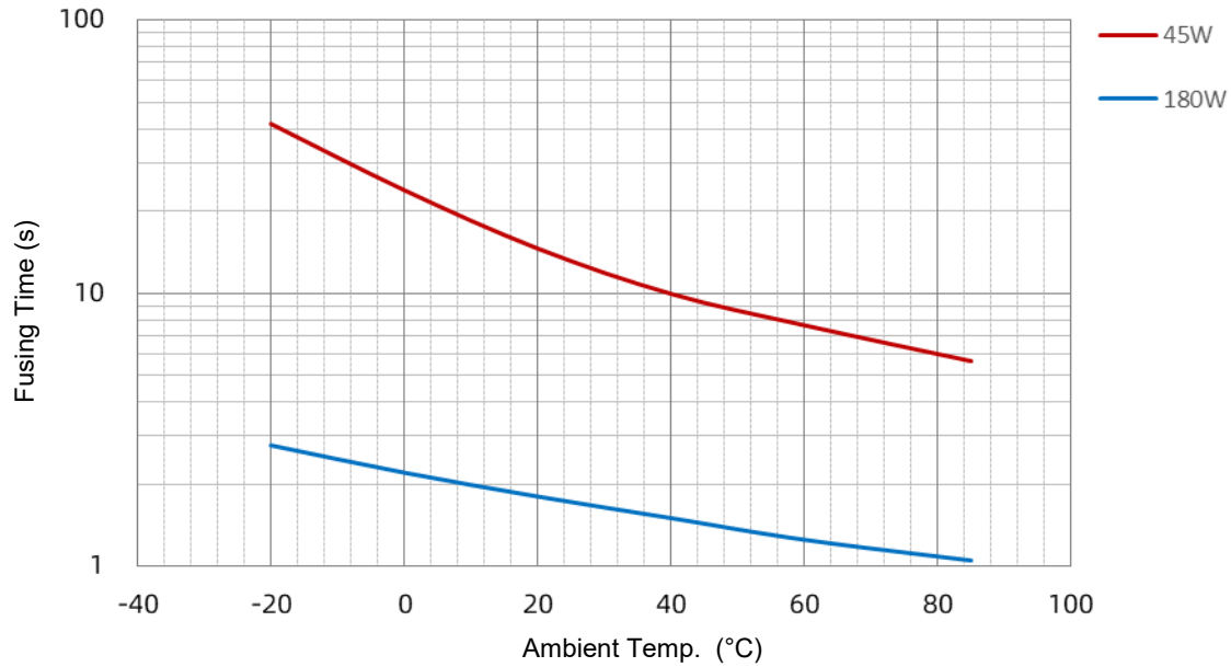
SKT-L 120 A Power-temp. curve
